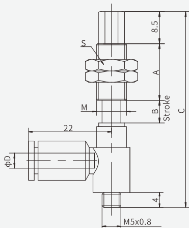
M5M Lateral rotating (one touch fitting)
