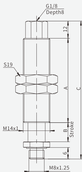
M8M Vertical rotating
